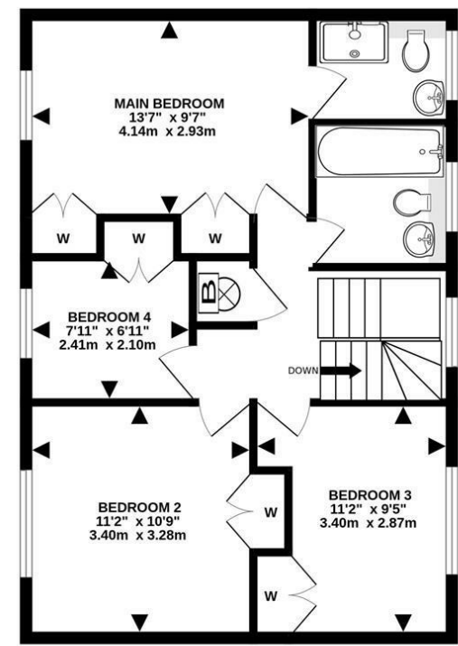
1ST FLOOR 596 sq.ft. (55.3 sq.m.) approx.
